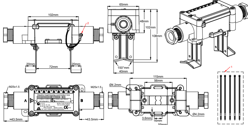
Example of mounting at distance of the pipe with the long legs stainless steel bracket (Mounting option 5)
