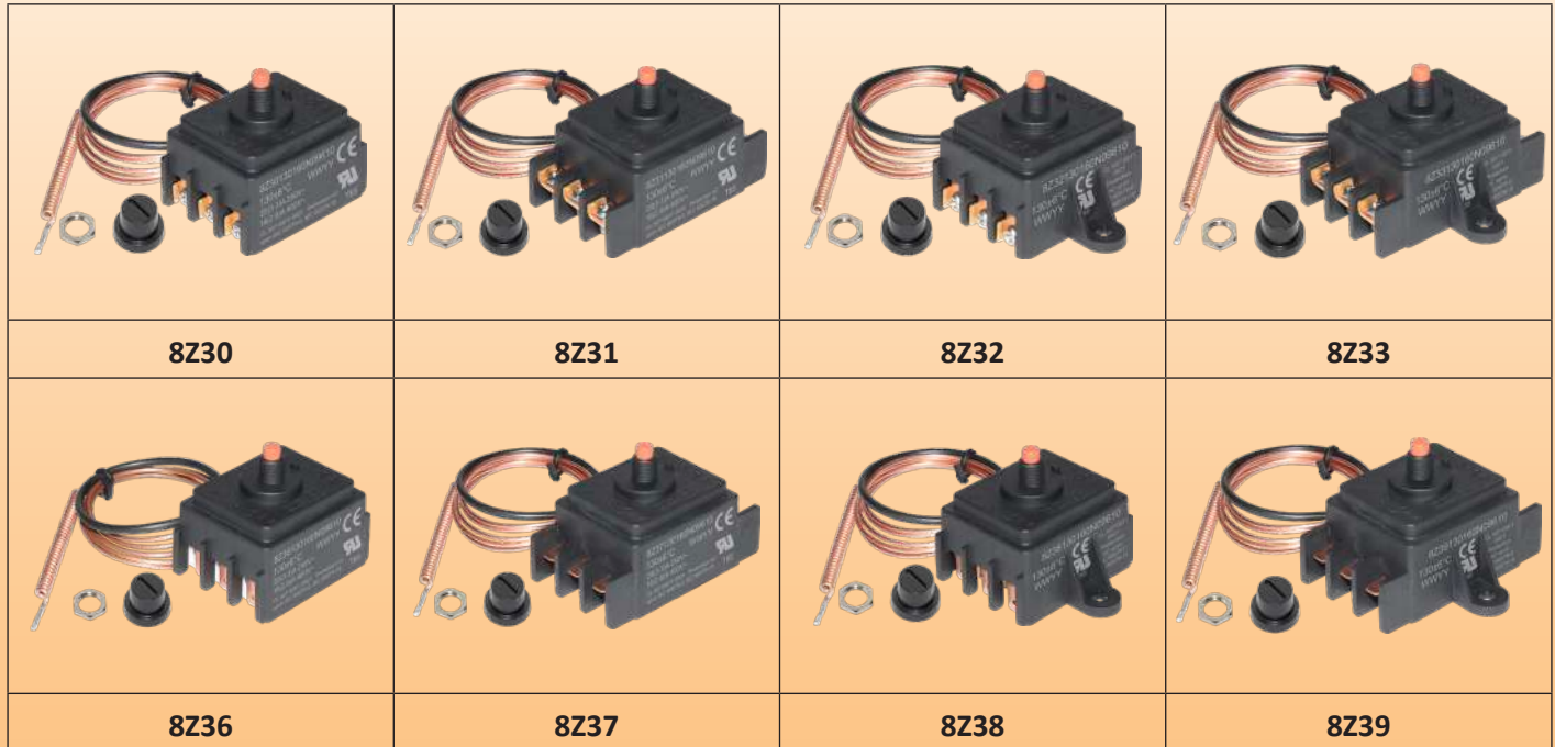
Mounting by M10×1 front bushing, vertical terminals (standard), type 8Z30 and 8Z36
